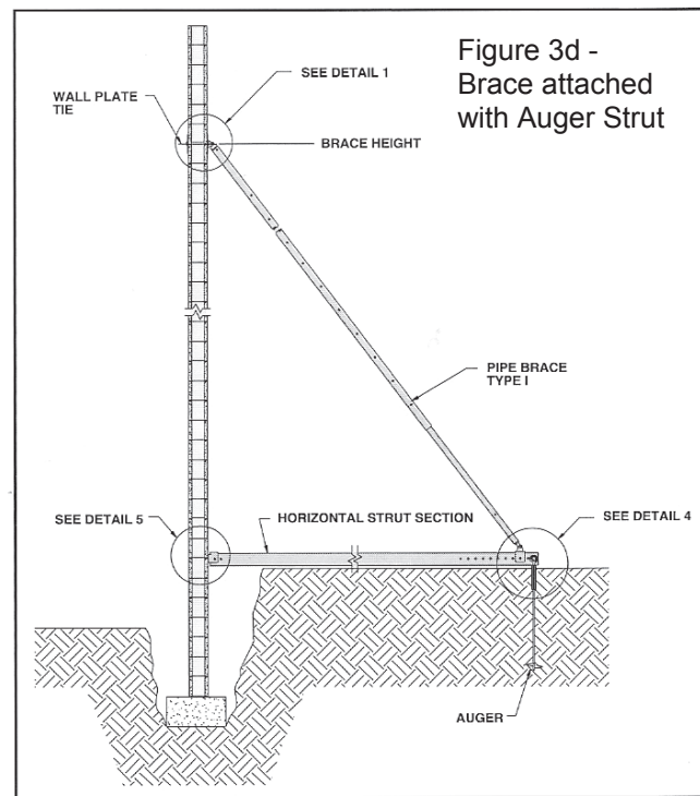
Figure 3 - Typical BRACE-RITE® SYSTEM CONFIGURATIONS
