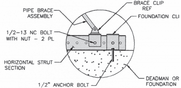
DETAIL 3
