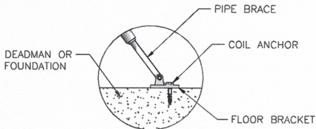
DETAIL 6
