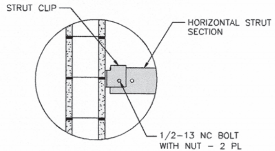
DETAIL 5
