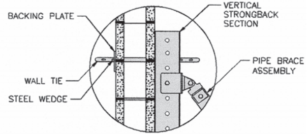
DETAIL 1A WITH STRONGBACK
