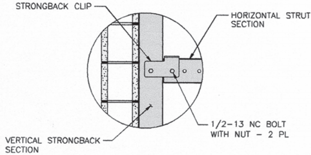
DETAIL 2
