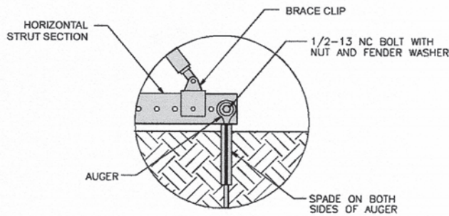
DETAIL 4
