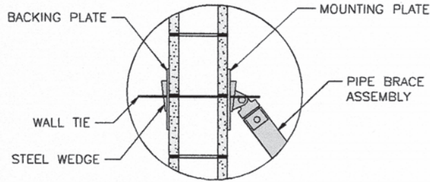
DETAIL 1 WITHOUT STRONGBACK
